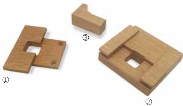
CABIDE 18_02.3 HANGER 100x100mm OAK
